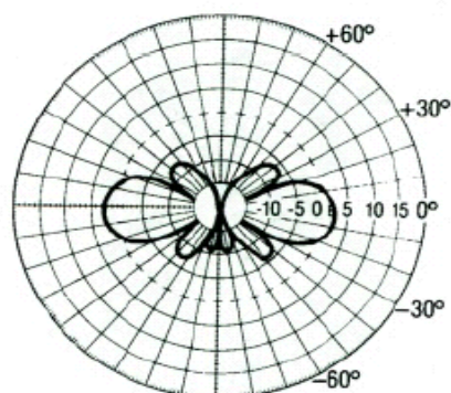
Diagrama de Radiación Vertical Vertical Radiation Pattern
